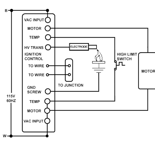
SCHEMATIC DIAGRAM
