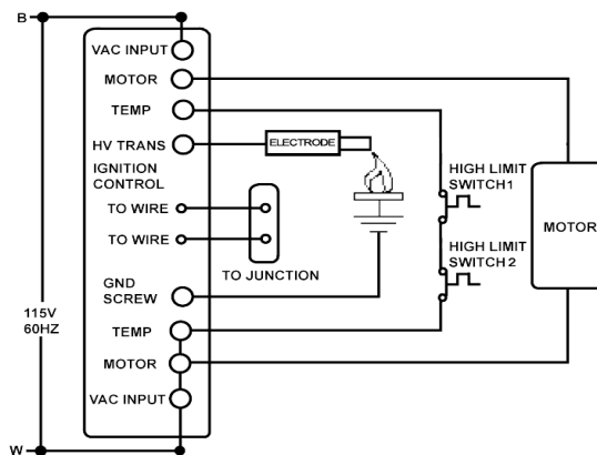
SCHEMATIC DIAGRAM
