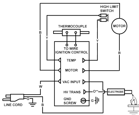
CONNECTION DIAGRAM
