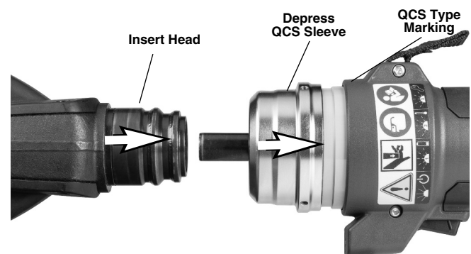
Figure 9 – Installing Interchangeable Head in the QCS Coupling
